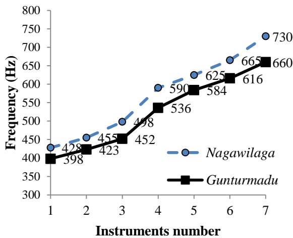
Fig. 3. Graph comparison of the fundamental frequency of gamelan Saron Ricik Nagawilaga and Gunturmadu.
