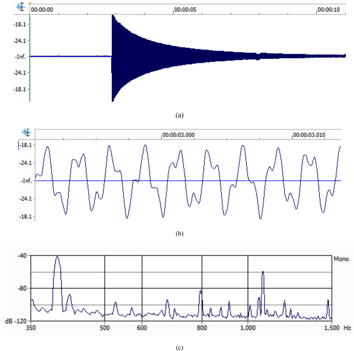
Fig. 2. Instrument #1 Gamelan Saron Ricik Gunturmadu (a) waveform as a function of time obtained instrument 1, (b) magnification of (a), and (c) as a function of the frequency spectrum (Fourier transform of the spectrum (a))
