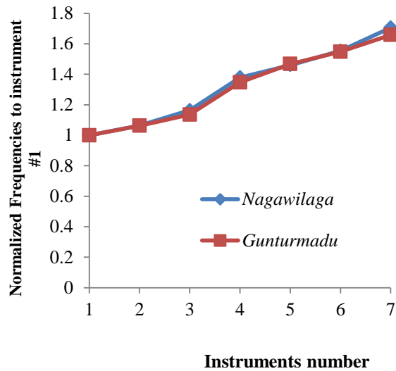
Fig. 4. Comparison of normalized frequencies and the fundamental frequency of instruments number 1 of Saron Ricik, Gamelan Nagawilaga and Gunturmadu
